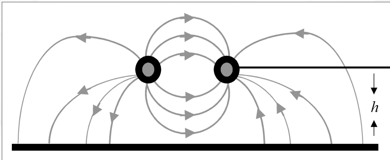
Figure 3: Common Mode Currents
