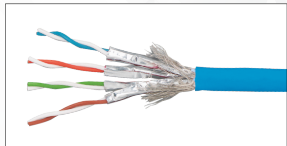
Figure 6: S/FTP Construction
