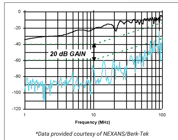
Figure 8: UTP VS. Ungrounded F/UTP Susceptibility
