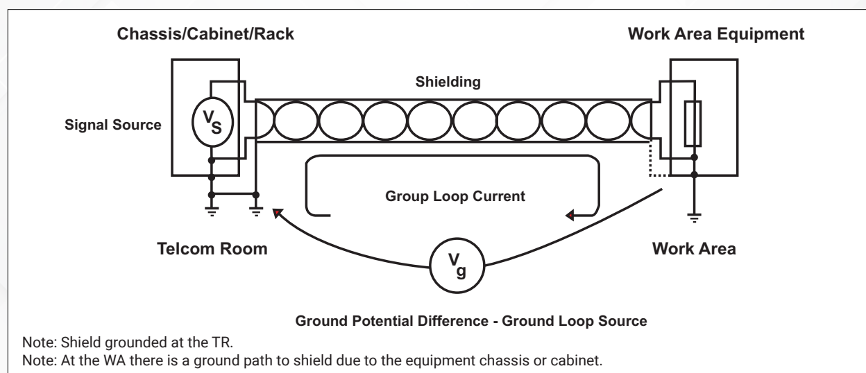
Figure 4: Introduction of Ground Loops
