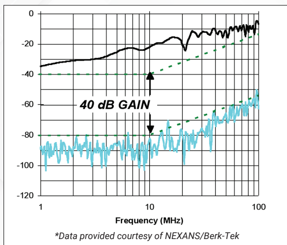
Figure 7: UTP VS. F/UTP Susceptibility
