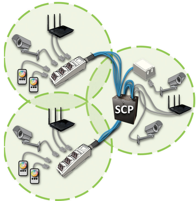
Figure 6: Example of building device connections in multiple coverage areas
