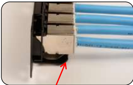
INTEGRATED GROUNDING STRIP CARRIES GROUND PATH FROM OUTLET TO PANEL WITHOUT ADDITIONAL WIRES
