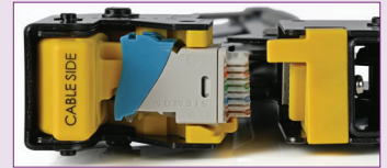
Hybrid Outlet
