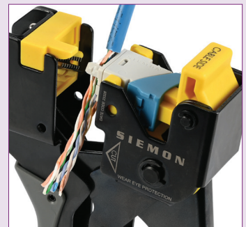
Panel Outlet
