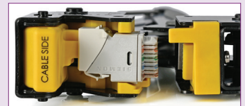
Keystone Outlet
