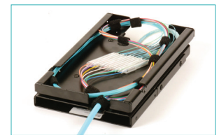
LightStack Mount Splice Enclosure
