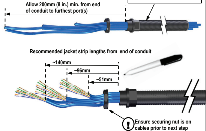
Measure, mark, & strip cables
