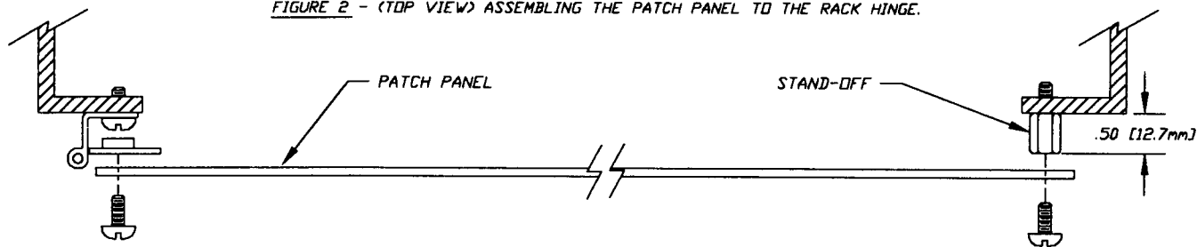
FIGURE 2 - (TOP VIEW) ASSEMBLING THE PATCH PANEL TO THE RACK HINGE.
