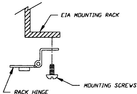
FIGURE 1 - (TOP VIEW) ASSEMBLING THE HINGE TO THE MOUNTING RACK.
