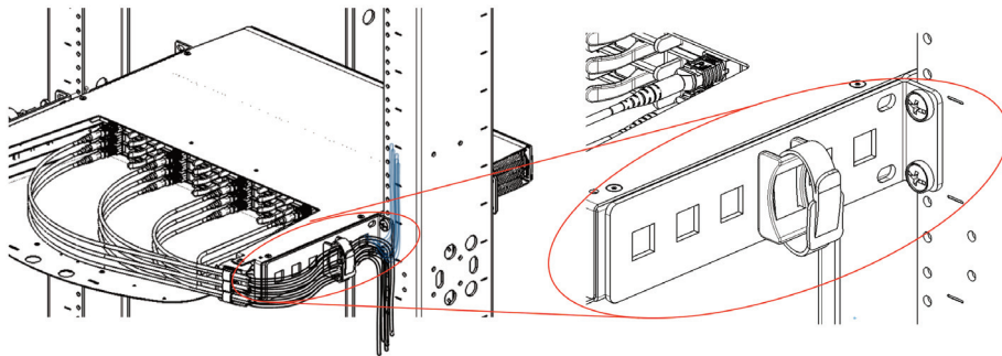
2 Post rack rear mount
