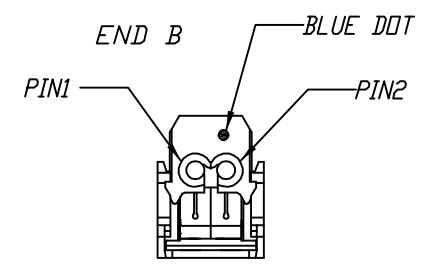
BACK VIEW OF UNTERMINATED PLUG
