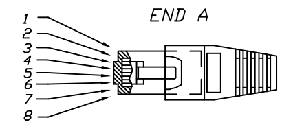
BACK VIEW OF UNTERMINATED PLUG
