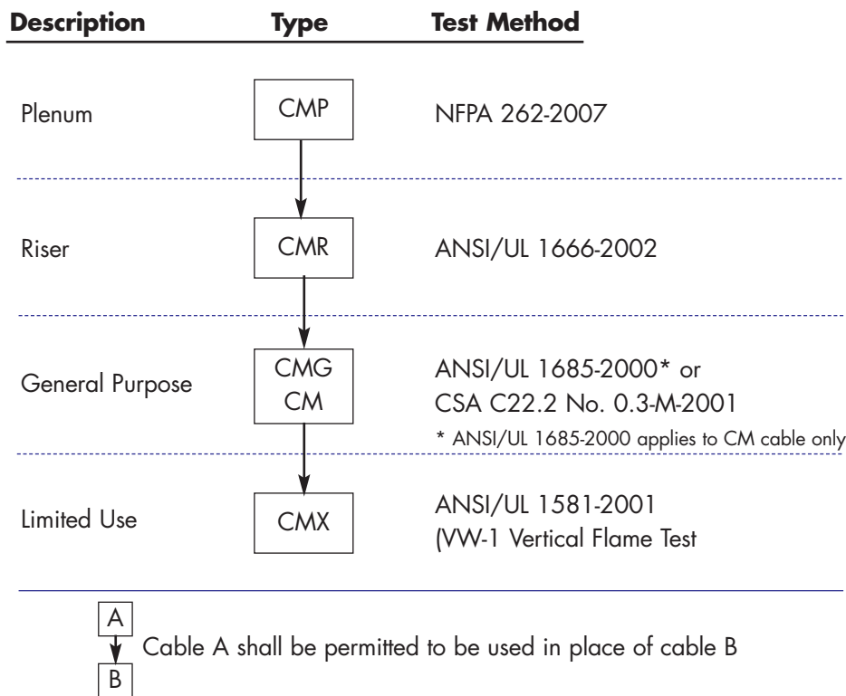
Figure 1: NEC Cable Substitution Hierarchy
