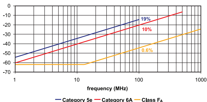
Figure 2: Comparative Channel PSACRF Coupling
