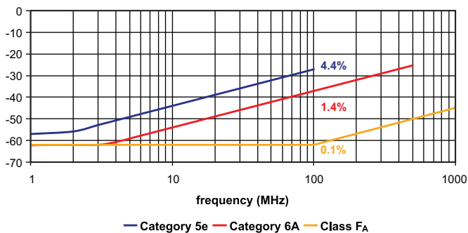
Figure 1: Comparative Channel PSNEXT Loss Coupling
