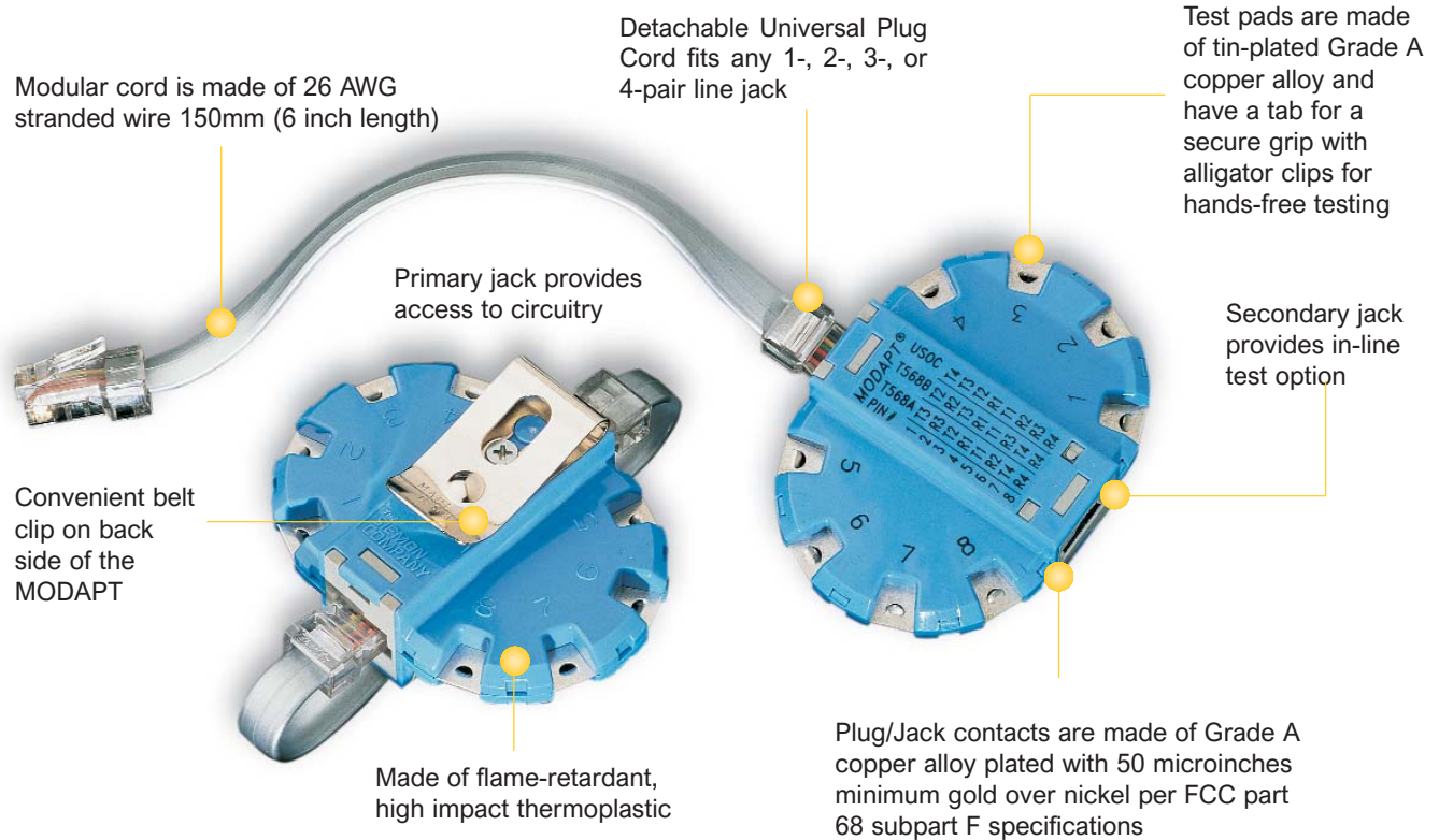
MODAPT.....Test adapter with one 152mm (6 in.) 4-pair universal plug-ended modular cord
