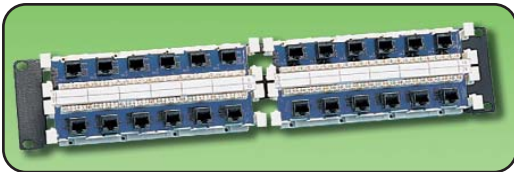
S110DB5-24RJP .....24-port jack panel, on a 19 inch panel, T568A/B wiring, 2 RMS
